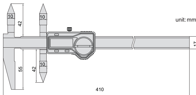
measure edge to hole center distance
