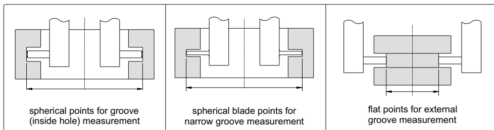
Measure internal and external grooves
