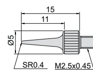
Needle Point
