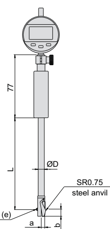
Range: 10-18mm
