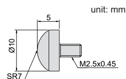
Spherical Point
