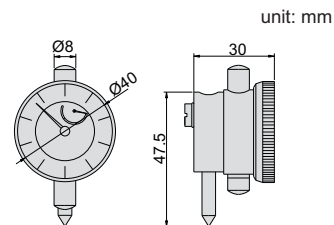
dial indicator
