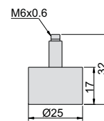
balance block
