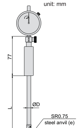
Range: 10-18mm
