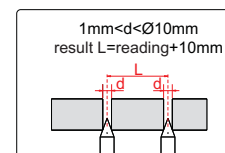
measure hole center distance
