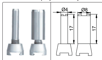
Clamps (included)
